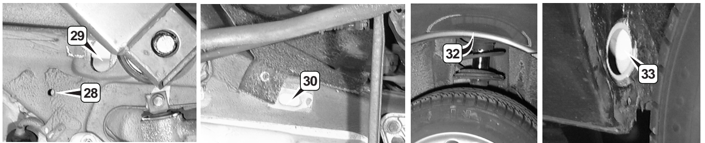
28. reinforcements at front end of floor panel
