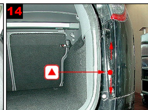
14 Rear wing: Treatment via 1 drill hole below tail light.
