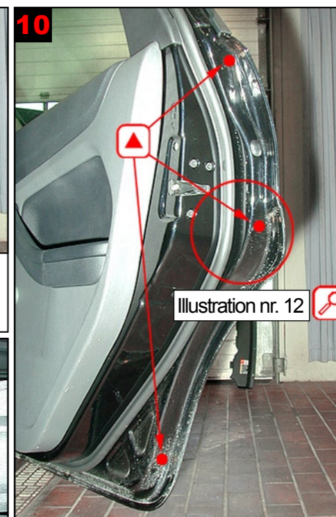
10 Rear door: 3 drill holes for correct treatment. See fig. 12 for correct drilling level.
