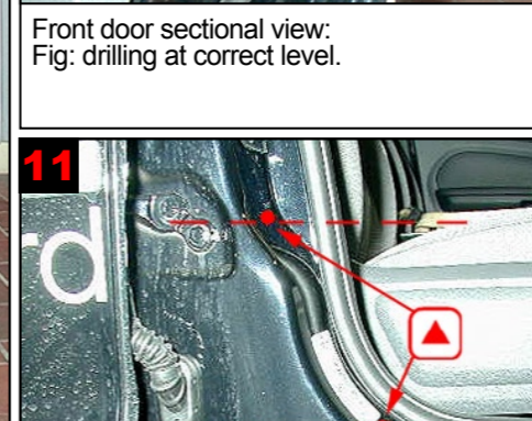
11 B-pillar: Drill 2 holes for correct treatment.
