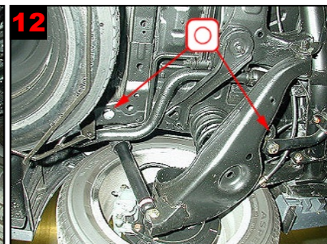
12 Longitudinal member in wheel arch rear: Treat via existing holes.
