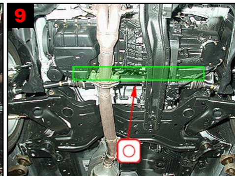
9 Cross member behind engine: Treat via existing holes.
