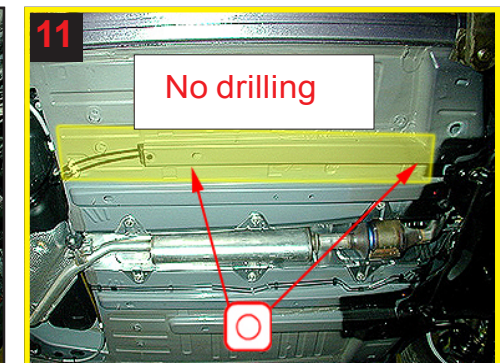
11 Longitudinal member centre right side. Treat via existing holes.
