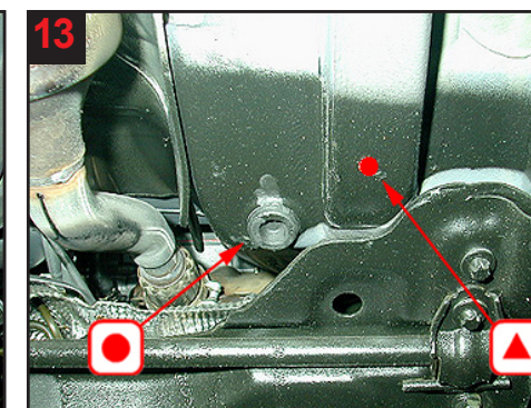
13 Longitudinal members by axle beam. Treat via 1 drilled hole and existing plug per side.
