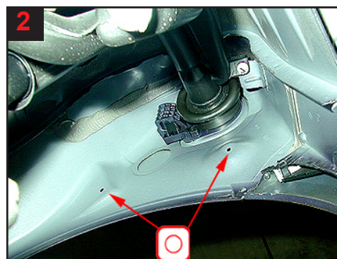
2 Wheel arch rear. Treat rear wing via 2 existing holes.
