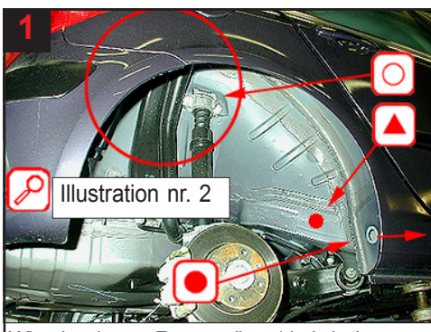
1 Wheel arch rear. Remove liner. 1 hole in the longitudinal member. Panels. Inject via existing plugged hole. Reinforcement for shock absorber via existing hole. See fig 2 for treating rear wing.
