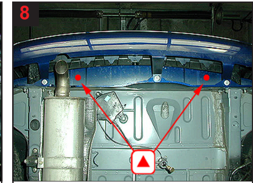
8 Rear panel/reinforcement for bumper. Treat via 2 drilled holes.
