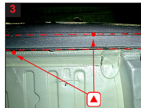
3 Panels. To drill into inner panel drill on the inside of the plate joint. To drill into outer panel drill on outer side of plate flange.
